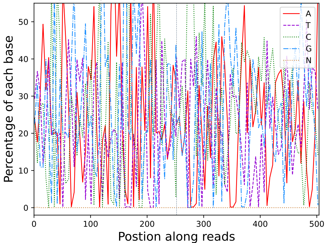
Base percentage along reads (R20209)
